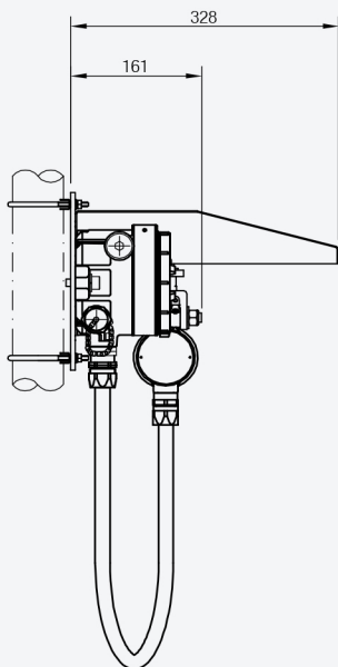
Pipe Mounted
