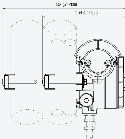
Pipe Mounted
