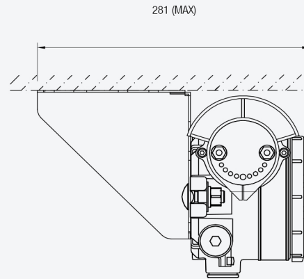
Ceiling Mounted
