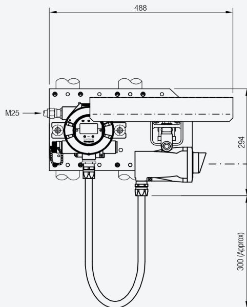
Pipe Mounted
