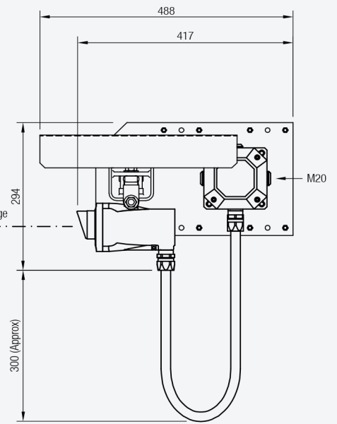
Surface Mounted
