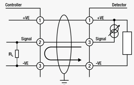
XCD Source Configuration
