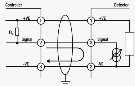
XCD Sink Configuration
