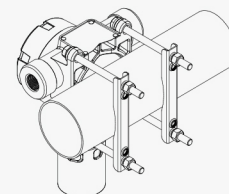
Vertical or horizontal pipe mounted (Using optional pipe mounting bracket)
